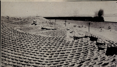
A long section of the Paotow-Lanchow line crosses desert. Foreground: straw squares to protect the track from moving sand dunes.
